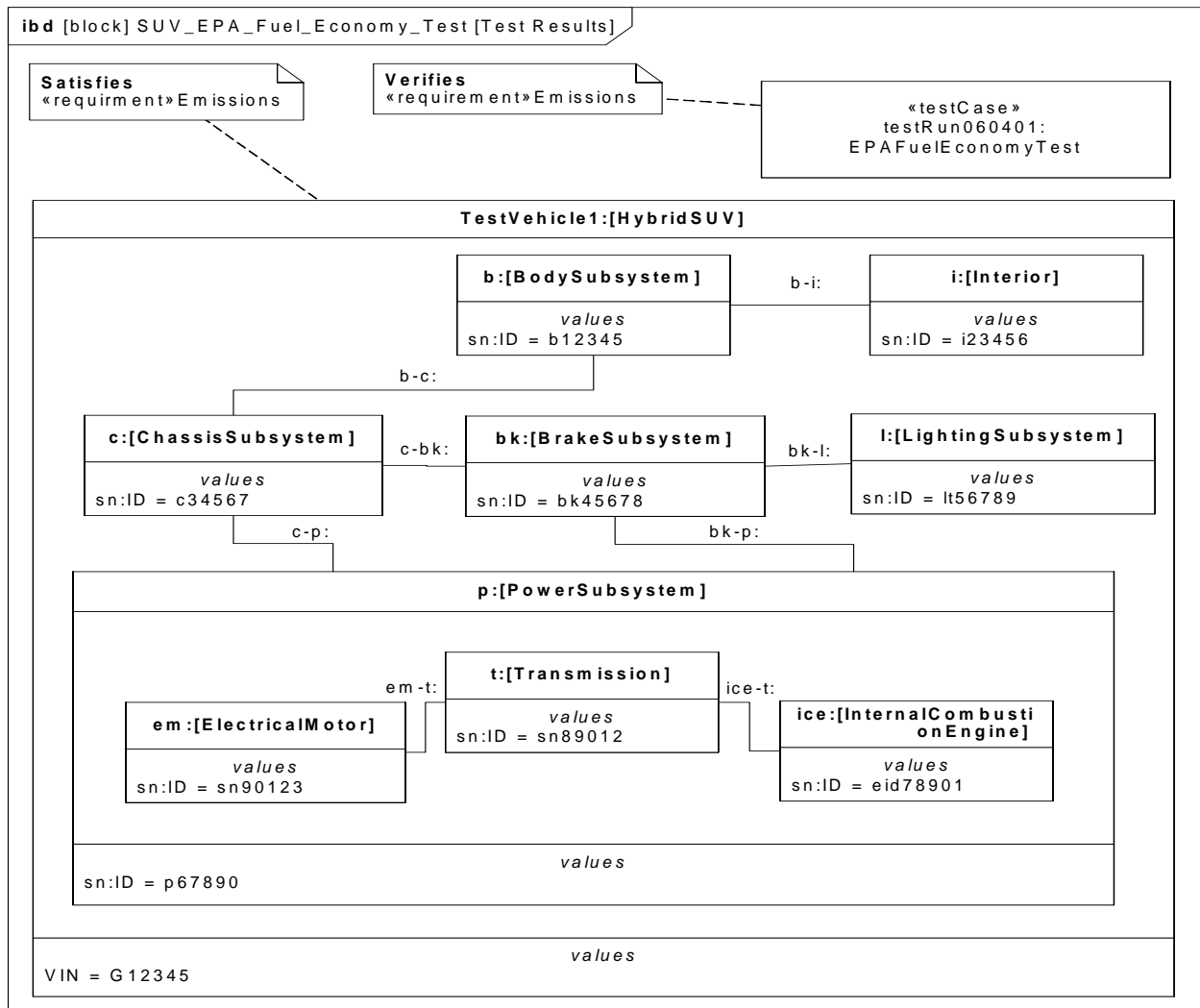
Figure B-38. Special Case of Internal Block Diagram Showing Reference to Specific Properties (serial numbers)
