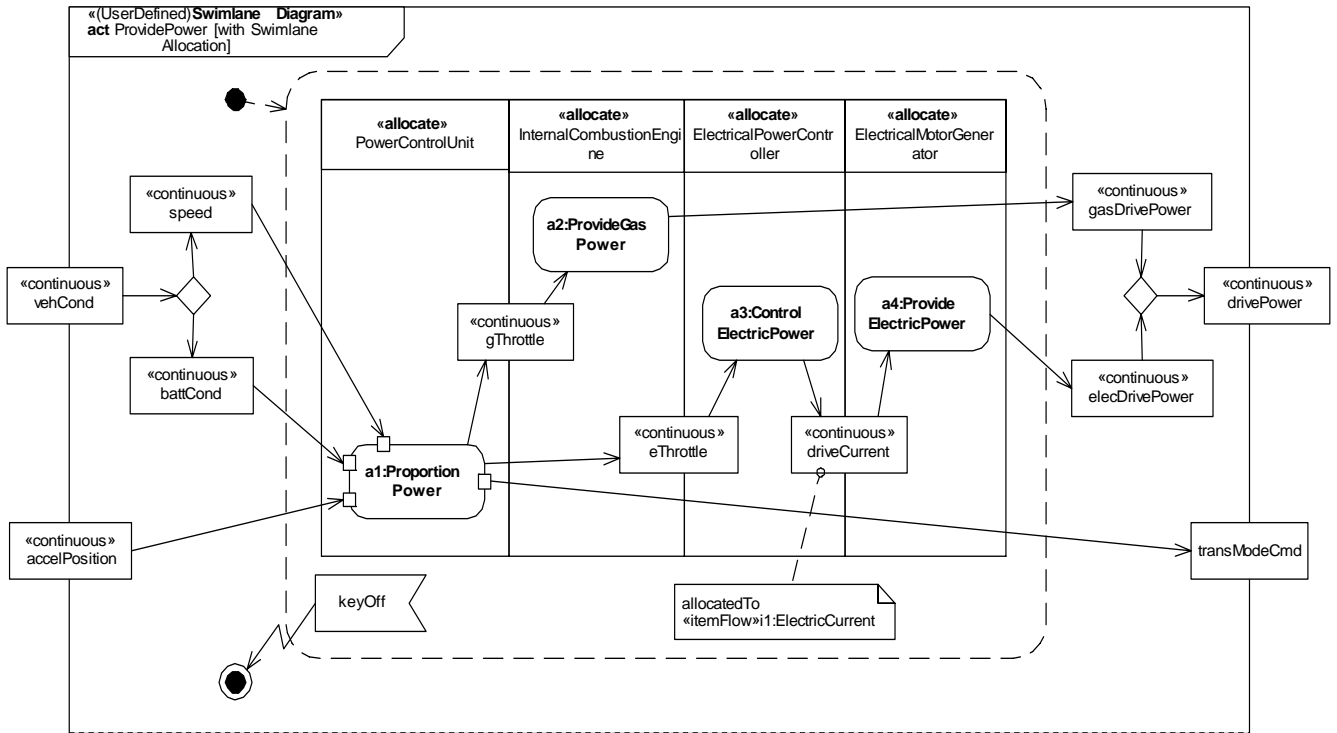
Figure 15-9. AllocateActivityPartitions (Swimlanes) for HybridSUV Cellarette Example
