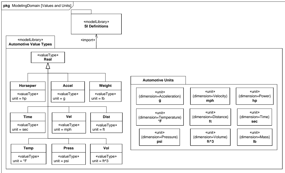
Figure B-2. Defining valueTypes and units to be Used in the Sample Problem.
