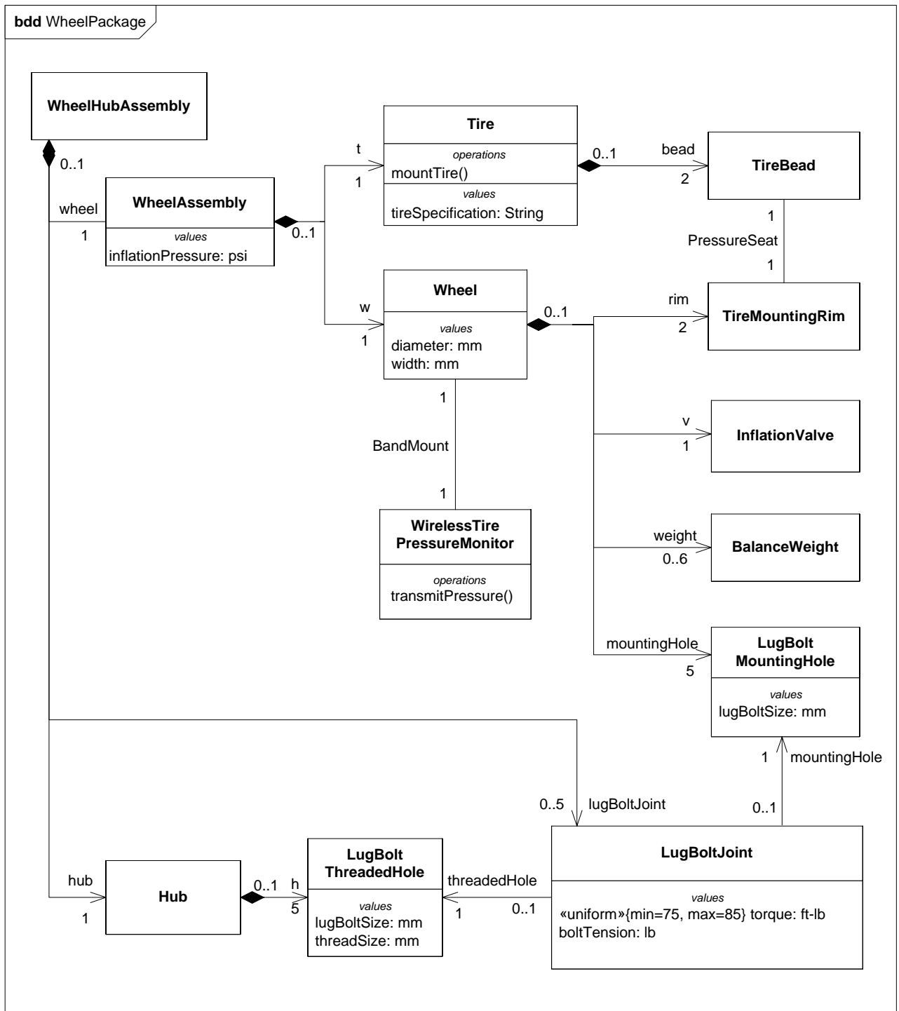
Figure 8-7. Block diagram for the Wheel Package
