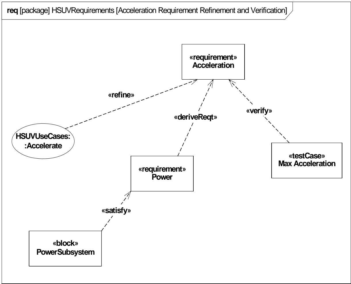
Figure B-13. Acceleration Requirement Relationships. (Requirements Diagram)
