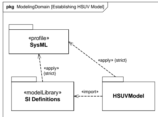
Figure B-1. Establishing the User Model by Importing and Applying SysML Profile & Model Library. (Package Diagram)
