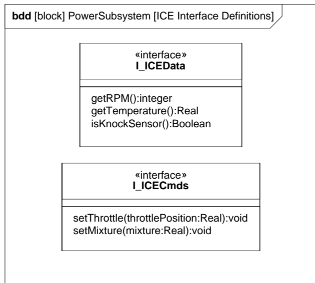
Figure 9-4. Interfaces of the Internal Combustion Engine ctrl Standard Port
