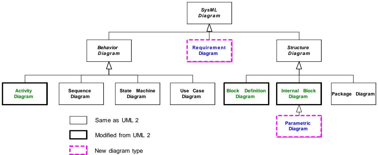
Figure 4-4. SysML Diagram Taxonomy
