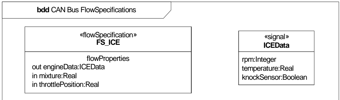
Figure 9-7. Flow Specification for the InternalCombustionEngine flow port to allow its connection over the CAN bus
