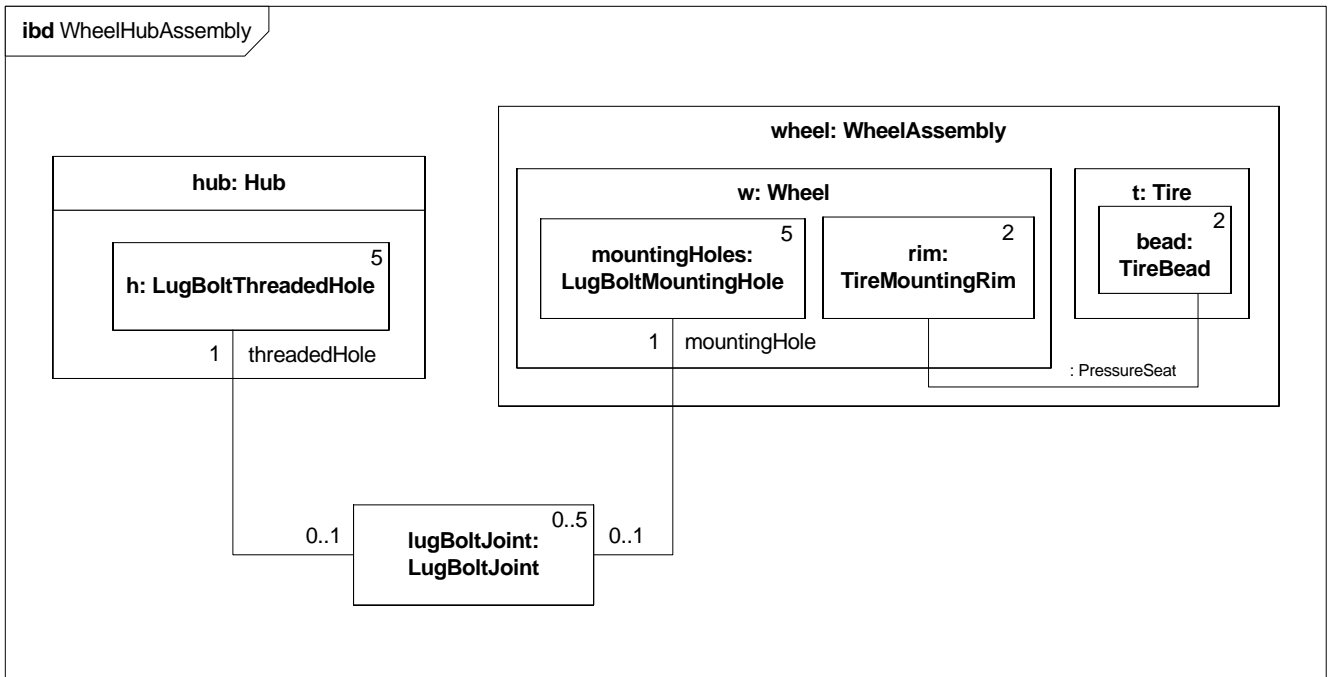
Figure 8-8. Internal Block Diagram for WheelHubAssembly
