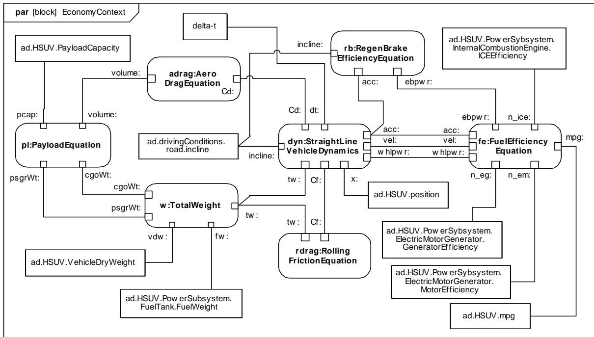
Figure 10-3. Constraints on a parametric diagram.
