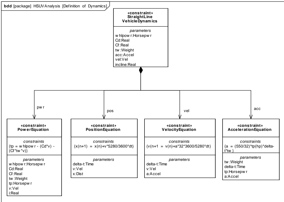
Figure 10-2. Constraint block definitions in a Block Definition diagram.
