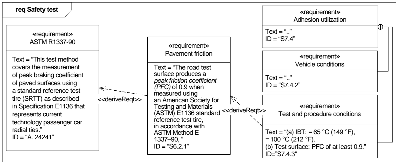
Figure 16-3. Requirements Derivation
