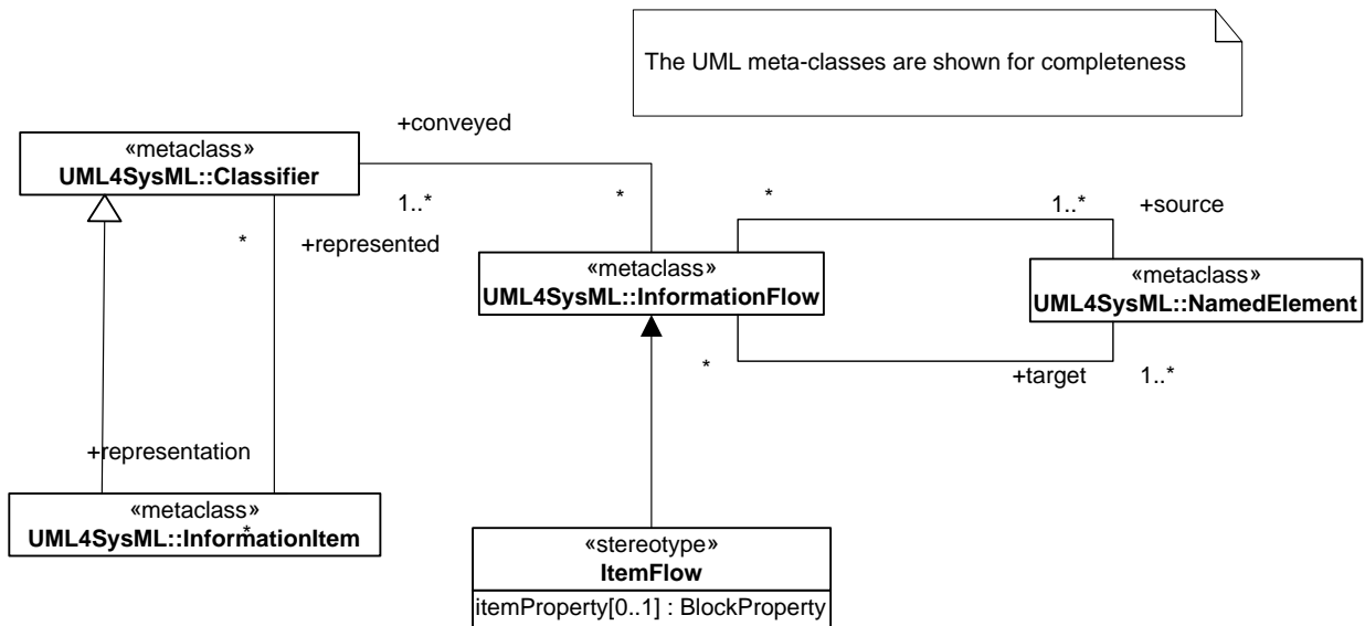
Figure 9-2. ItemFlow Stereotype
