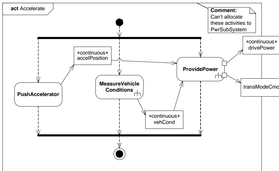
Figure B-33. Behavior Model for “Accelerate” Function. (Activity Diagram)
