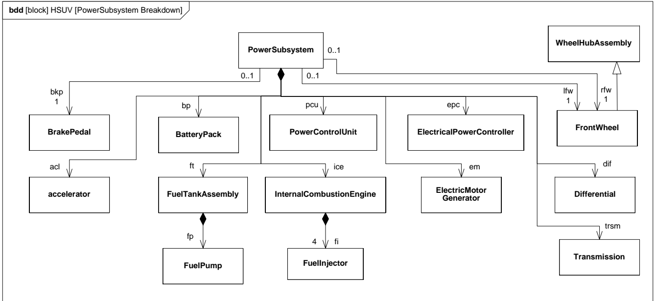
Figure B-18. Defining Structure of Power Subsystem (Block Definition Diagram)
