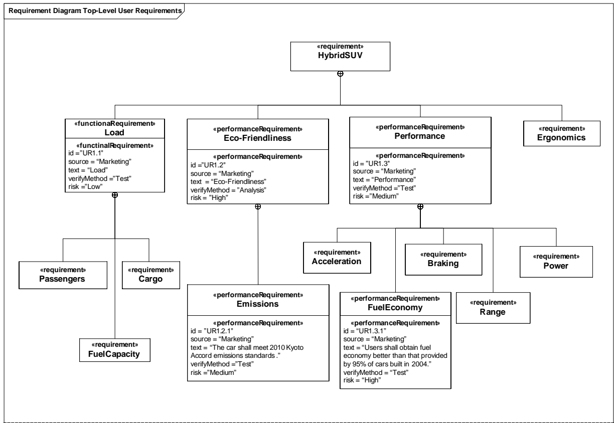
Figure C-3. Example extensions to Requirement
