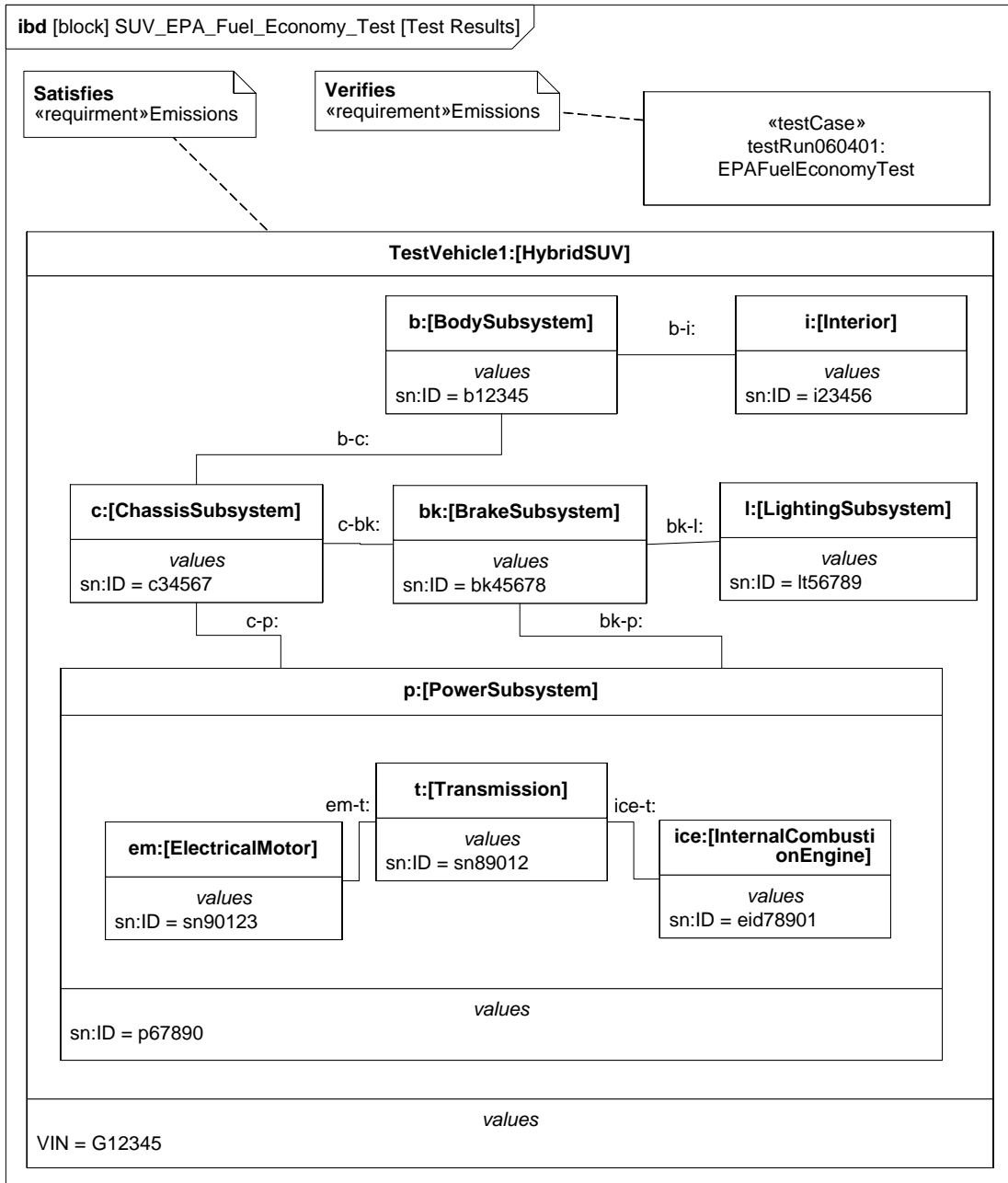
Figure 8-10. SUV EPA Fuel Economy Test
