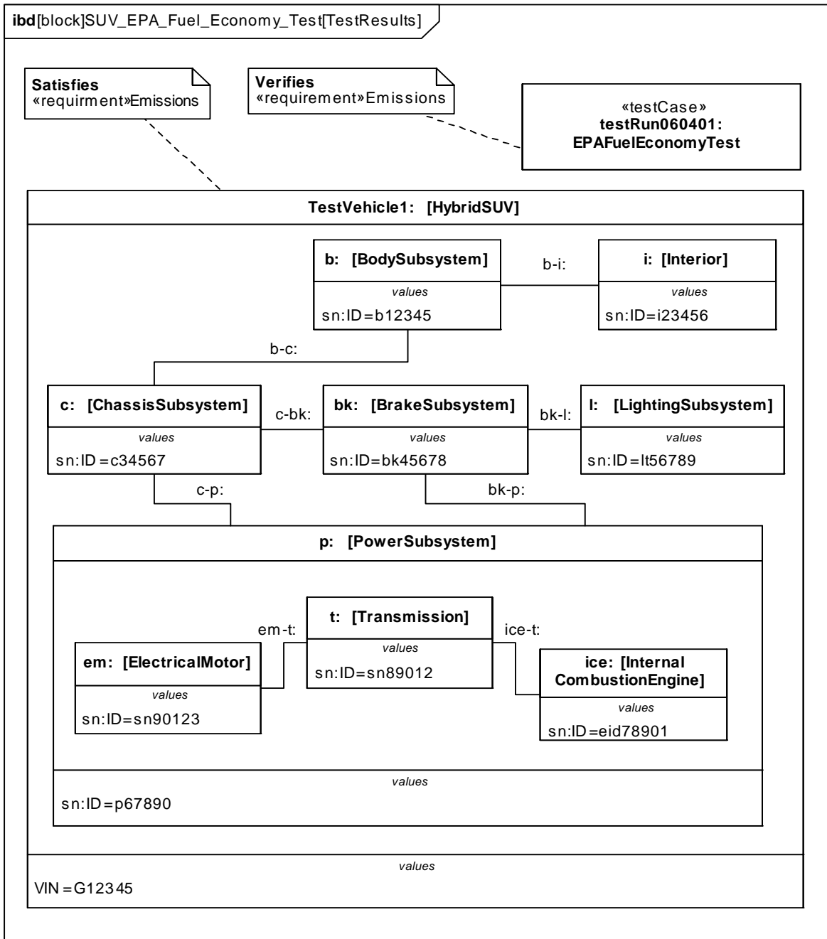
Figure B.38 - Special Case of Internal Block Diagram Showing Reference to Specific Properties (serial numbers)
