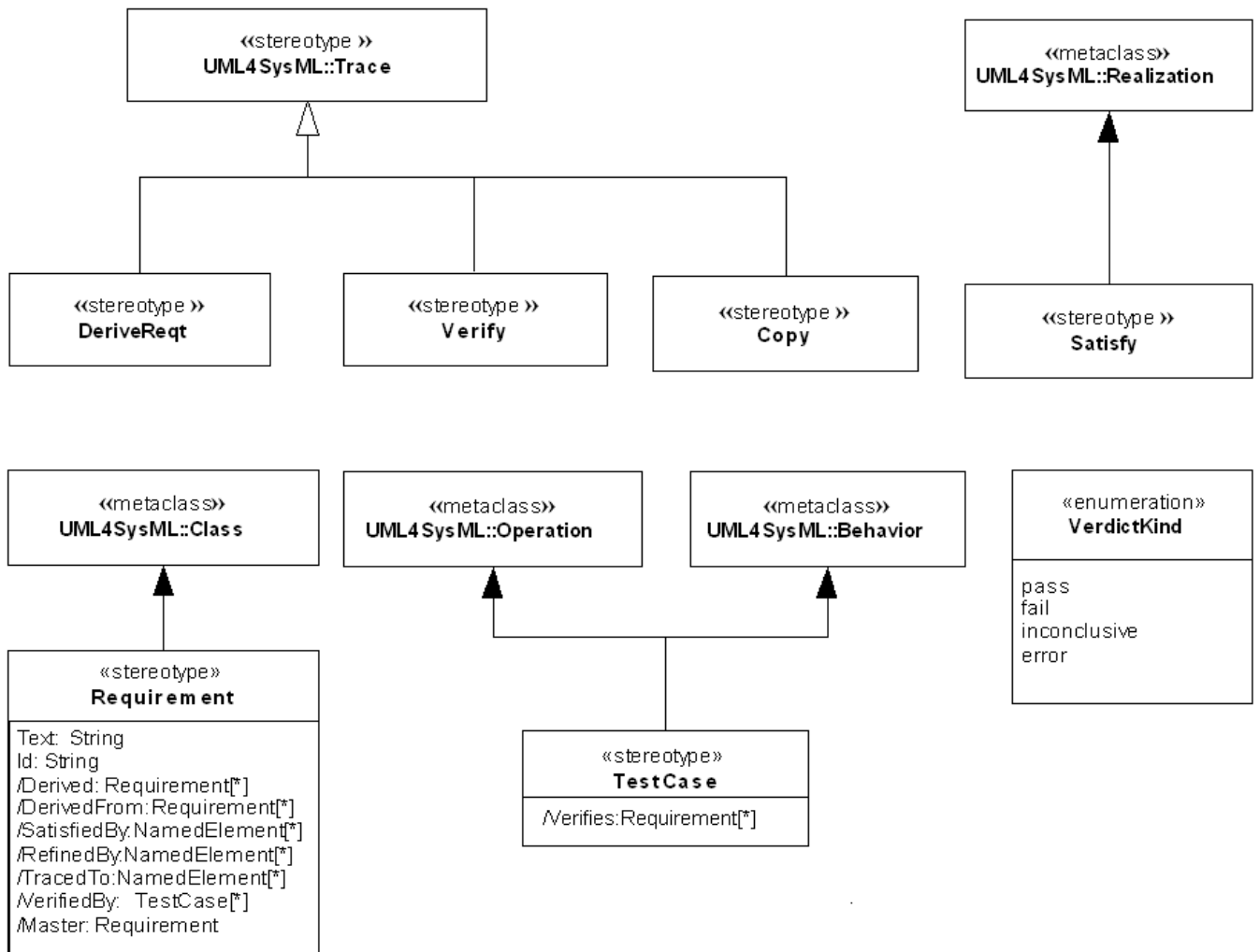
Figure 16.1 - Abstract Syntax for Requirements Stereotypes
