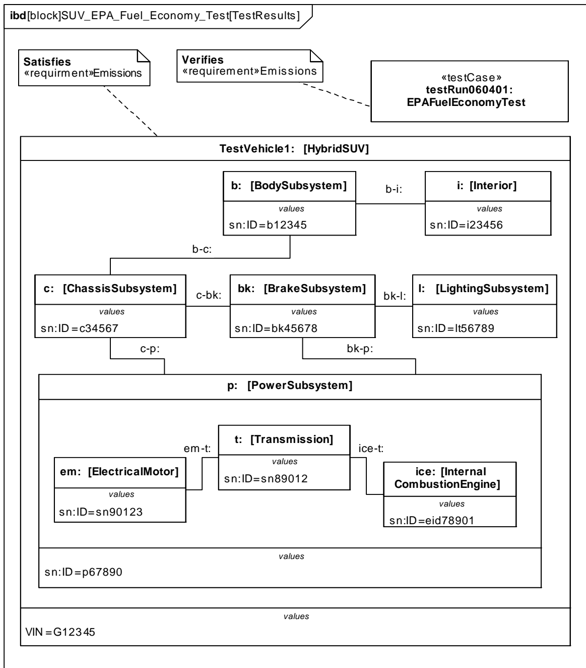
Figure 8.11 - SUV EPA Fuel Economy Test
